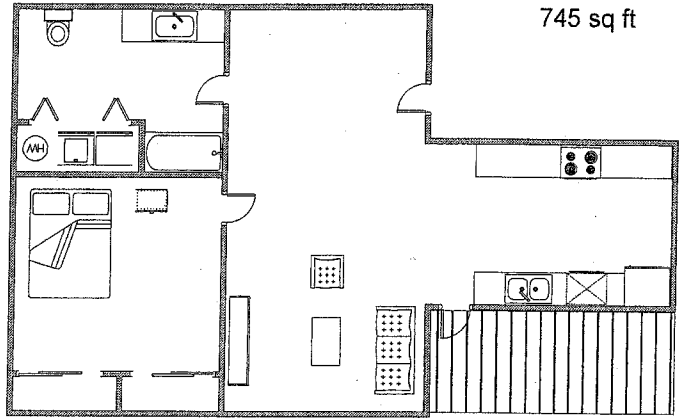
Two Bedroom Unit Floor Plan E 930 sq ft
